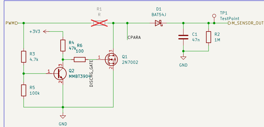
Capacitive soil sensor 125KHz
